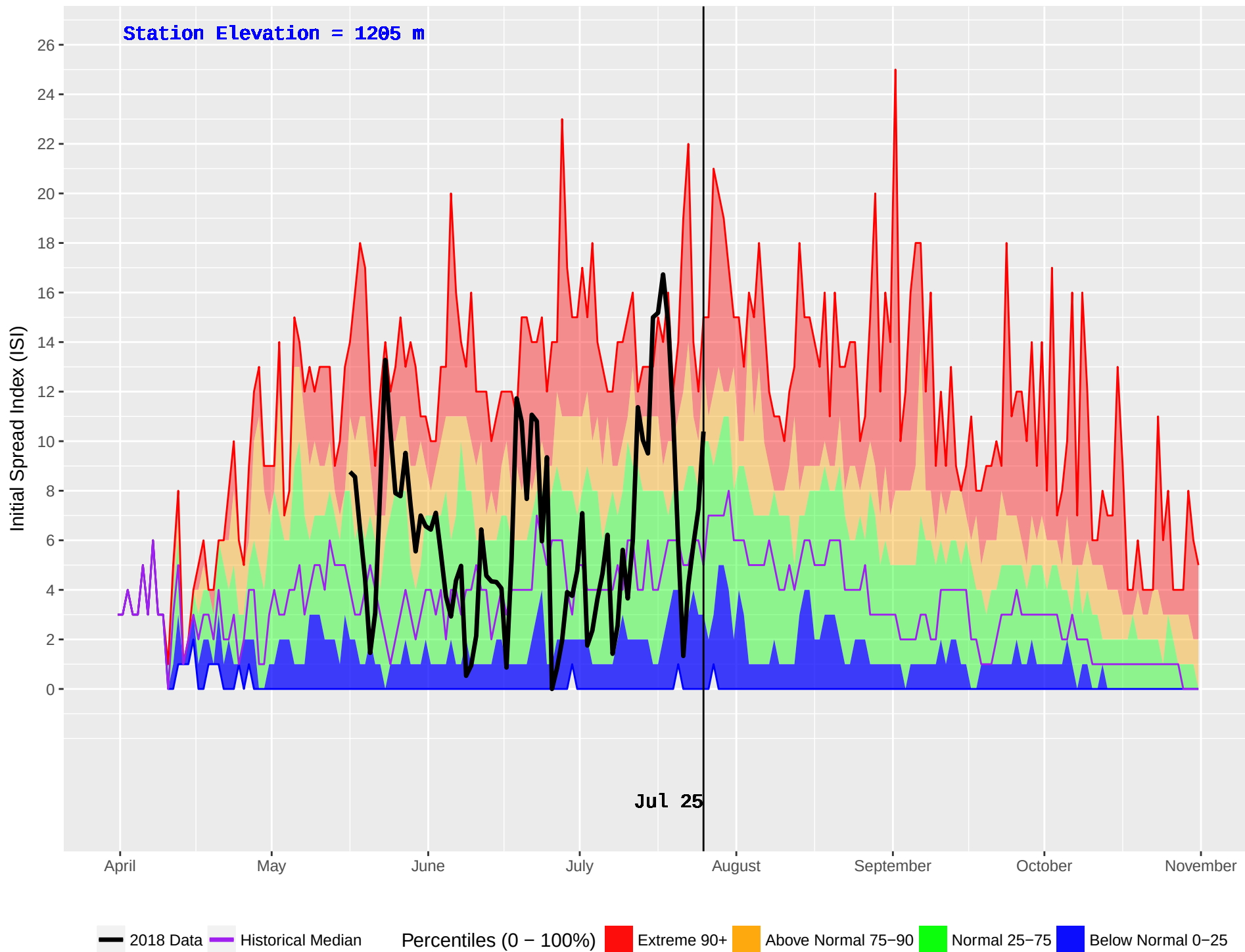
GWYNETH LAKE (309) : Historical (1986–2016) and Current (2018) Noon Initial Spread Index (ISI)
